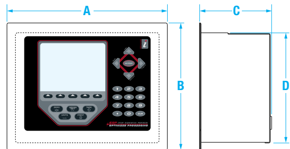
920i Panel Mount Dimensions
